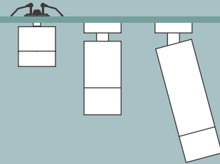
Surface Adjustable
